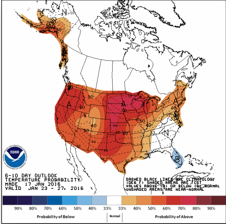
Temperature Probability
