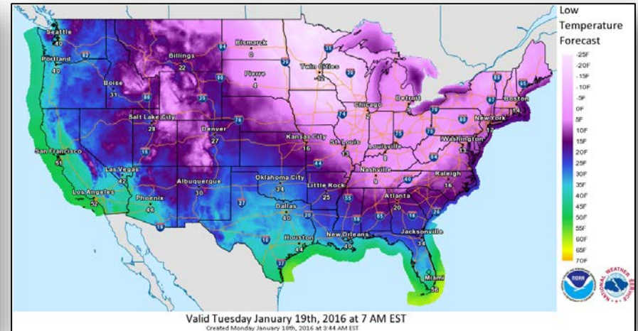
Low Temperatures
