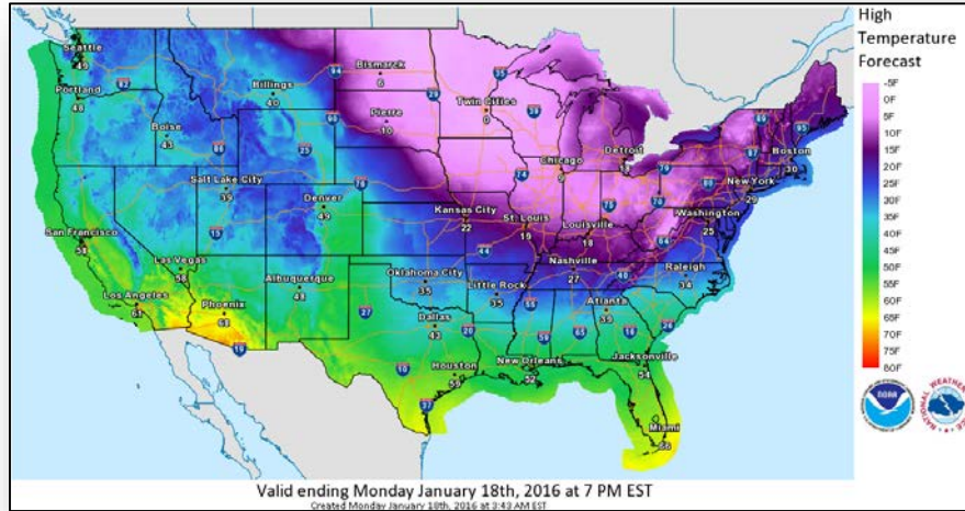
High Temperatures
