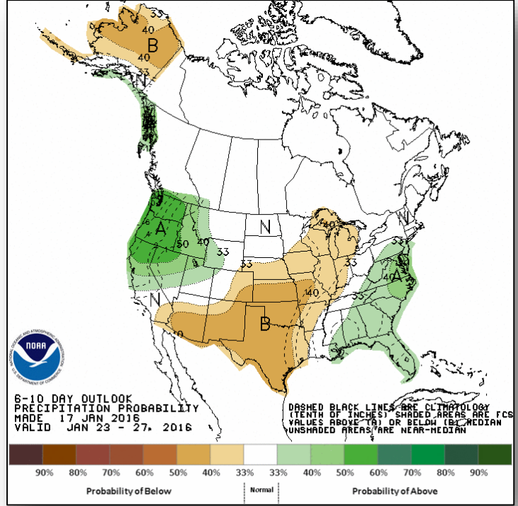
Precipitation Probability
